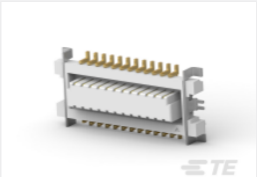
TE Part #1775013-2 0.8 BTB FS RCPT G/F 24P
