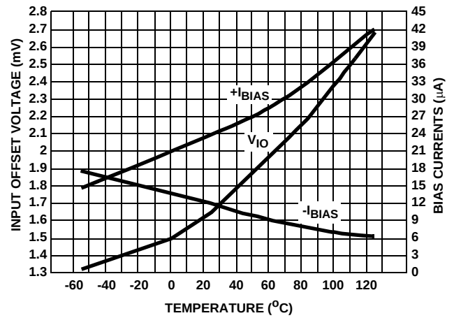
FIGURE 24. V_{\text{IO}} AND BIAS CURRENTS vs TEMPERATURE
