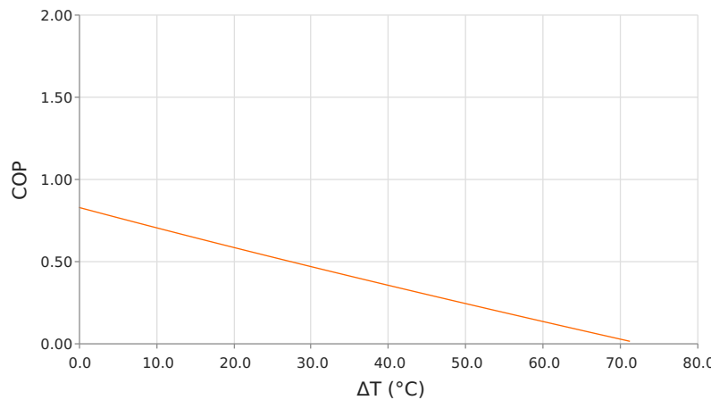
Coefficient of Performance ( COP = Q_c/P_{in} ) T_{hot} = 35\text{ }^{\circ}\text{C} | operating = 1.8 Amps
