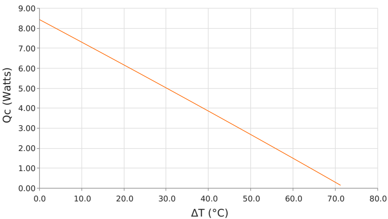
Heat Pumped at Cold Side ( Q_c ) T_{hot} = 35\text{ }^{\circ}\text{C} | operating = 1.8 Amps
