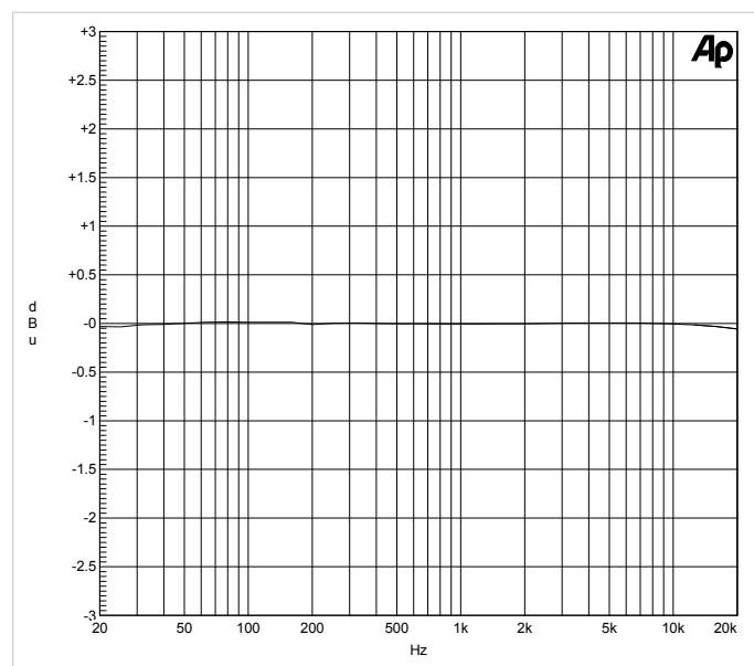
Z4II/Z8II Music Output Frequency Response
