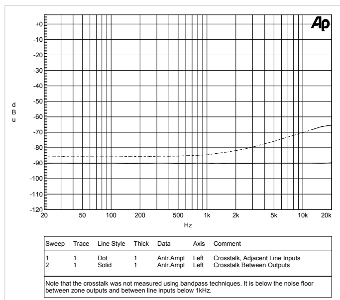
Z4II/Z8II Music Crosstalk
