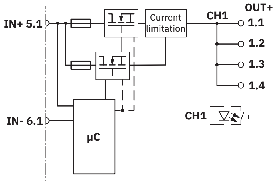
Block diagram
