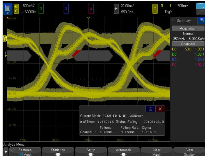
Figure 10. CAN FD eye-diagram mask testing.
