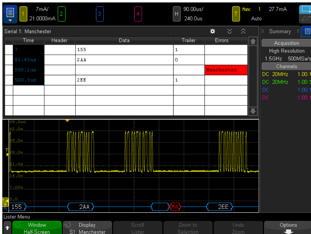
Figure 7. PSI5 decode on an InfiniiVision X-Series oscilloscope.
