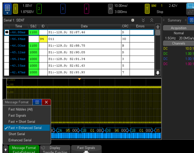
Figure 6. SENT decode on an InfiniiVision X-Series oscilloscope.
