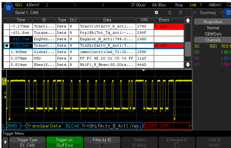
Figure 3. CAN decode on an InfiniiVision X-Series oscilloscope.
