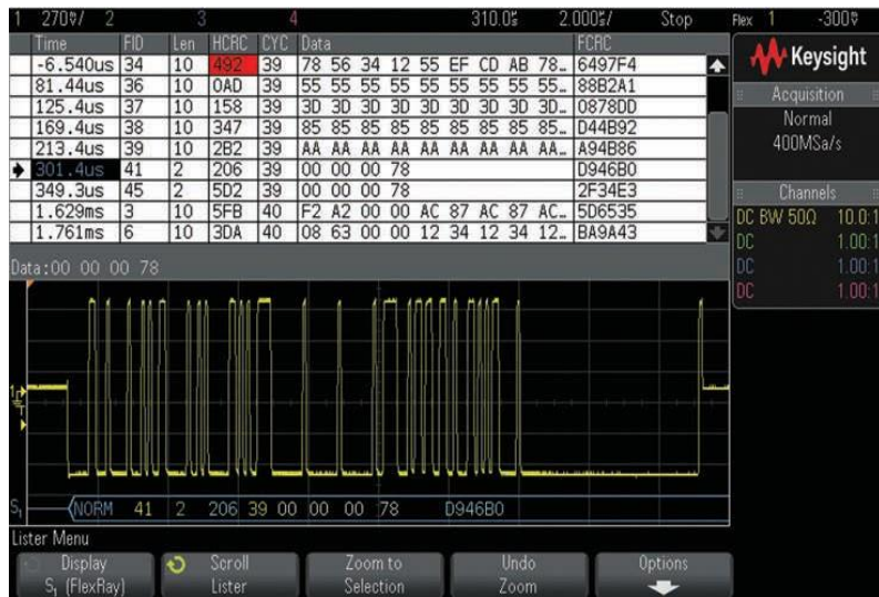
Figure 5. FlexRay decode on an InfiniiVision X-Series oscilloscope.
