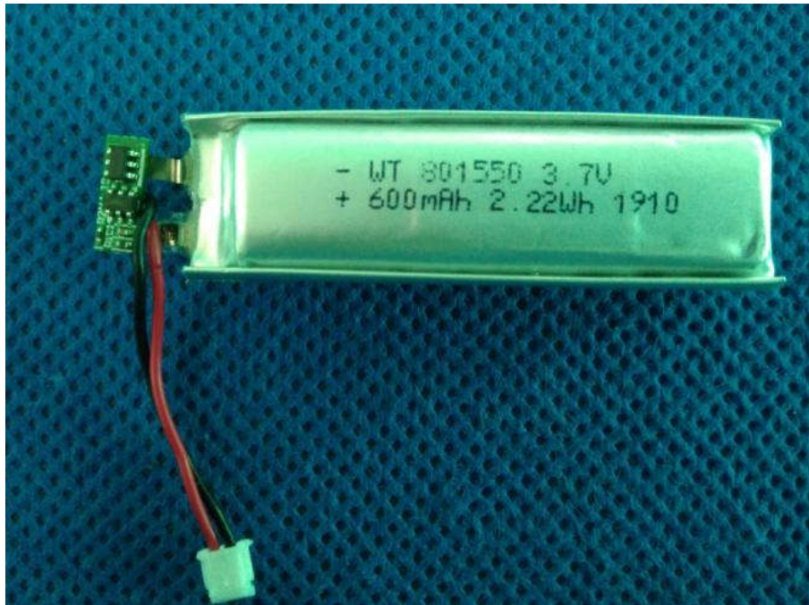
电池内部结构 Battery internal structure
