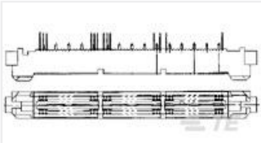
TE Part #2327671-2 RECEPT ASSY, RA, 84 POS, SLIVER 2.0
