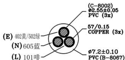
X-X CROSS-SECTION
