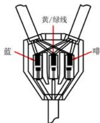
压接装配图纸
