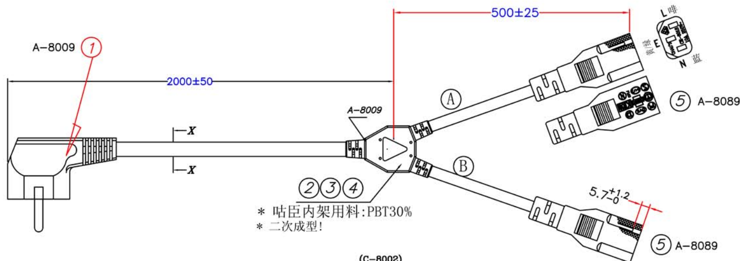
压接装配图纸
