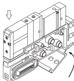
Figure. Block mounting procedure
