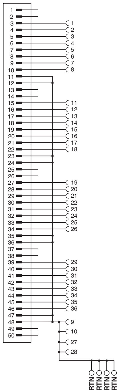
Circuit diagram
