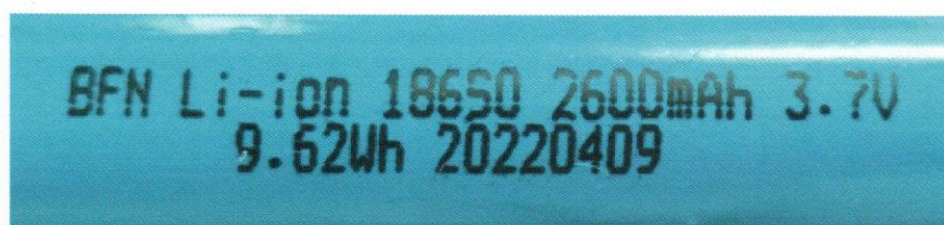
电池组铭牌 View of the battery nameplate
