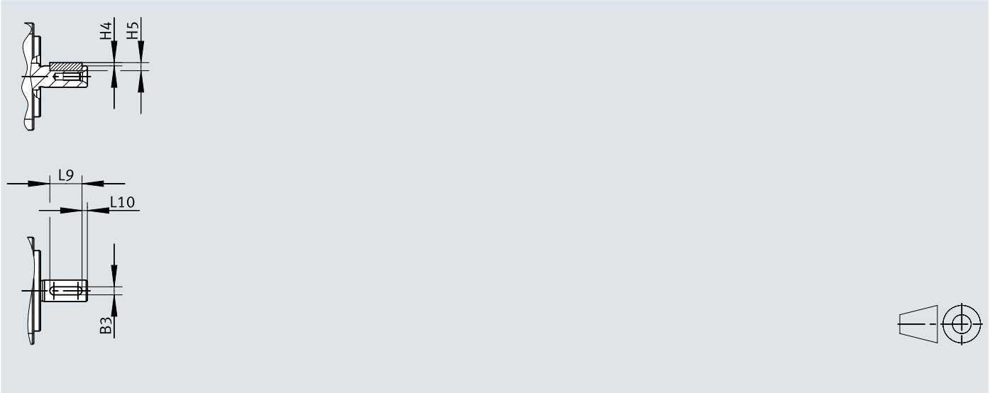
Dimensions – Featherkey for EMMT-EC-40
