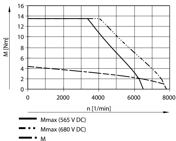
Torque M as a function of rotational speed n for EMMT-AS-80, very long, high voltage, without/with brake
