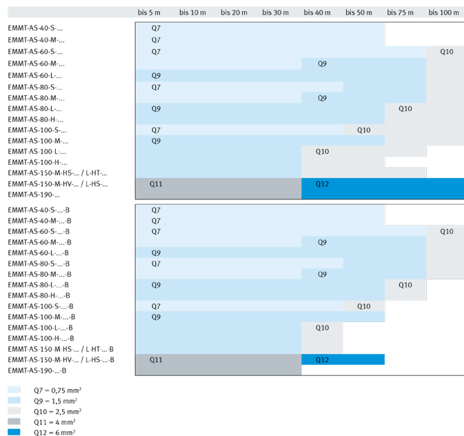
Recommended cable cross-section as a function of cable length and servo drive CMMT-AS
