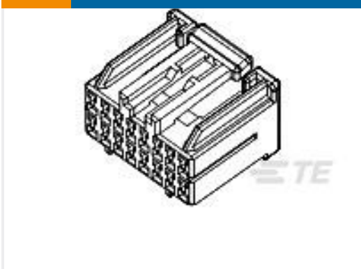
TE Part #917978-6 HYBRID MK-2 PLUG HSG ASSY 12P
