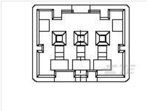
TE Part #1903392-1 GIC 2.5 W CAP HSG 3P NATURAL
