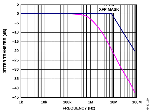
Figure 10. Jitter Transfer: OC-192 (TRANBW[2:0] = 3)
