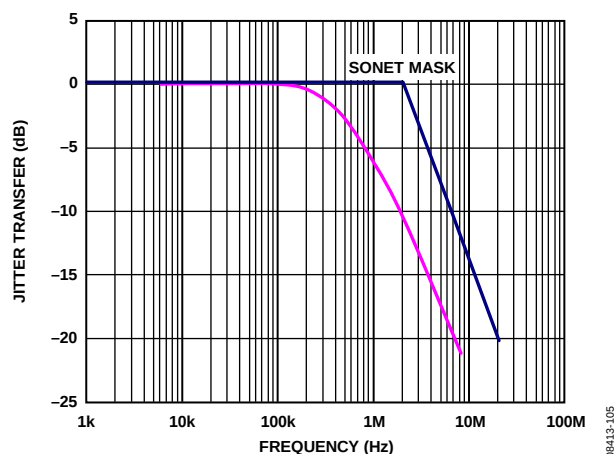
Figure 11. Jitter Transfer: OC-48
