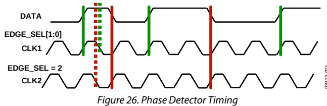
Figure 26. Phase Detector Timing
