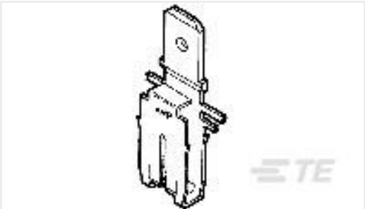
TE Part #63459-3 MAG-MATE 250 F-TAB 15-16 TPBR
