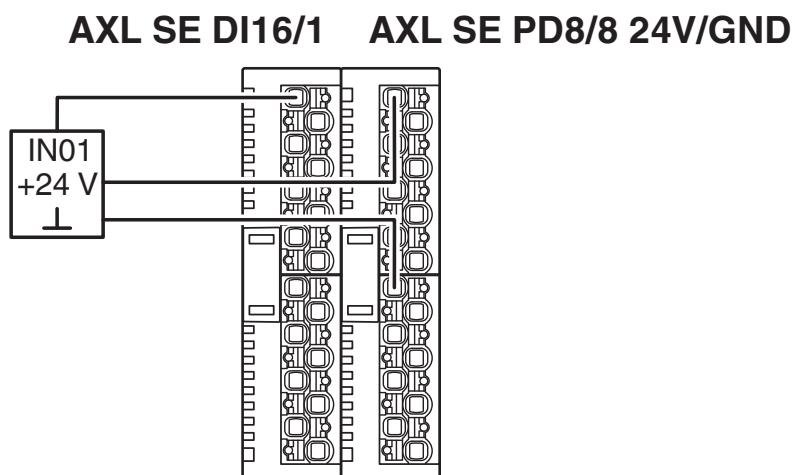
Connection diagram
