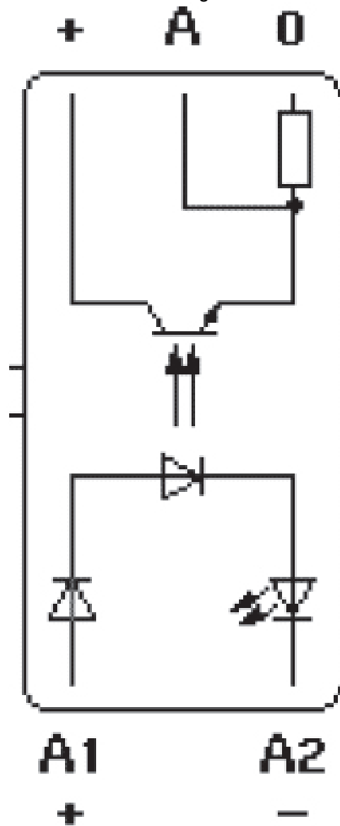
Circuit diagram
