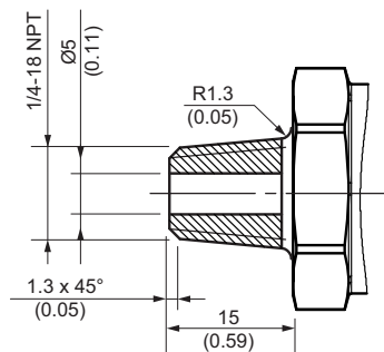
1/4"-18 NPT (male)
