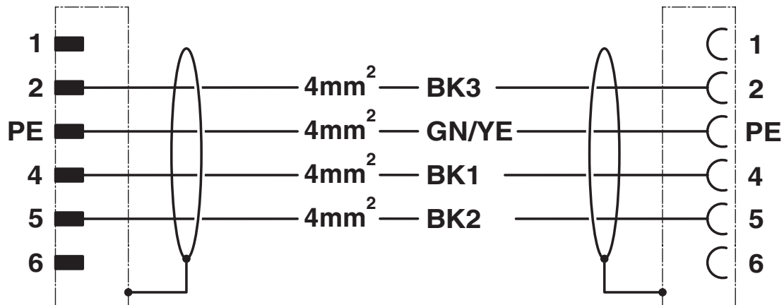
Contact assignment of M23 plugs/sockets
