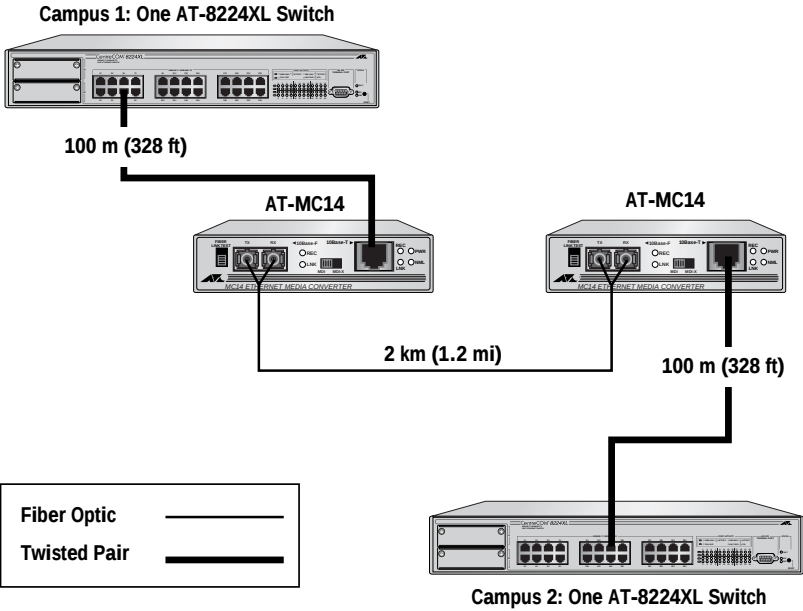
Figure 6 Back-to-Back Topology
