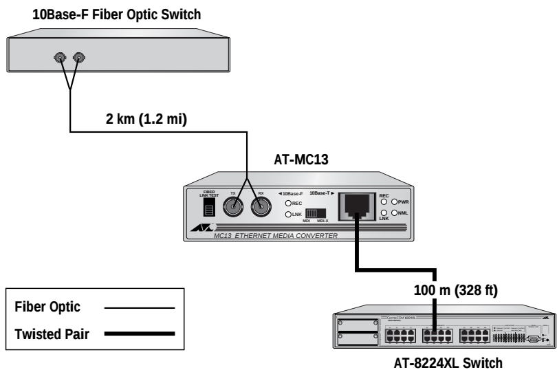
Figure 5 Standalone Topology
