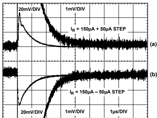
Figure 21. Transient Settling
