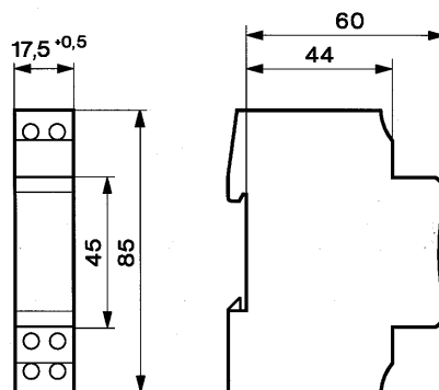
Dimensional details
