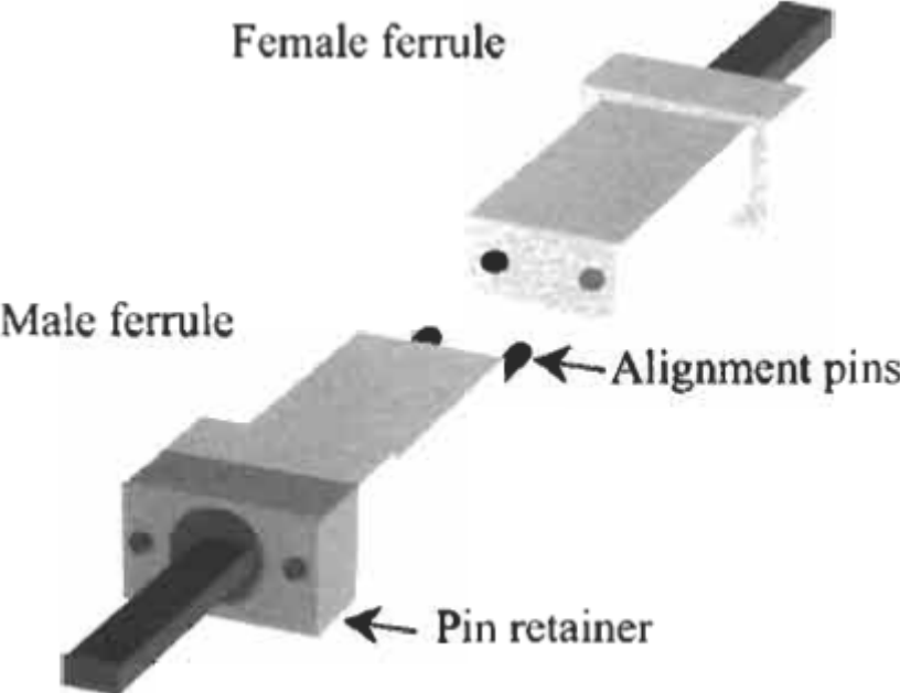
Fig. 3.2 MT-RJ ferrule alignment method.
