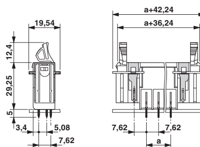
Dimensioned drawing
