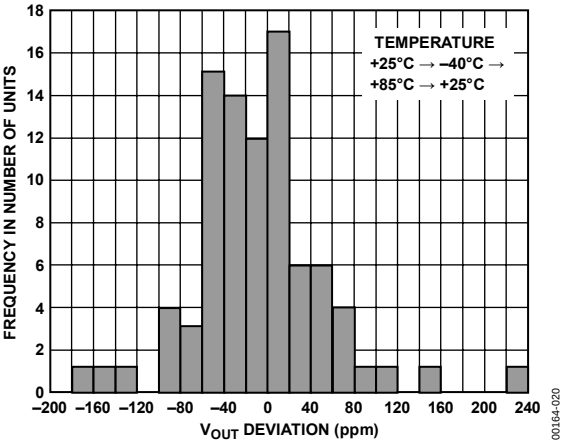
Figure 20. Typical Hysteresis for ADR29x Product
