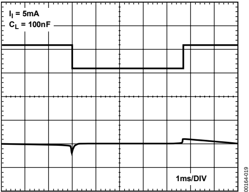
Figure 19. Load Transient
