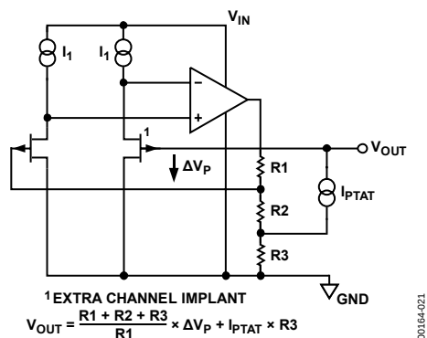
Figure 21. Simplified Schematic
