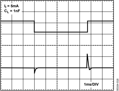
Figure 18. Load Transient
