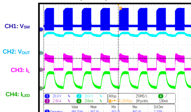
PWM Dimming f_{PWM} = 2kHz ( D = 0.5 )
