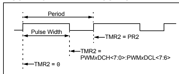
FIGURE 19-1: PWM OUTPUT
