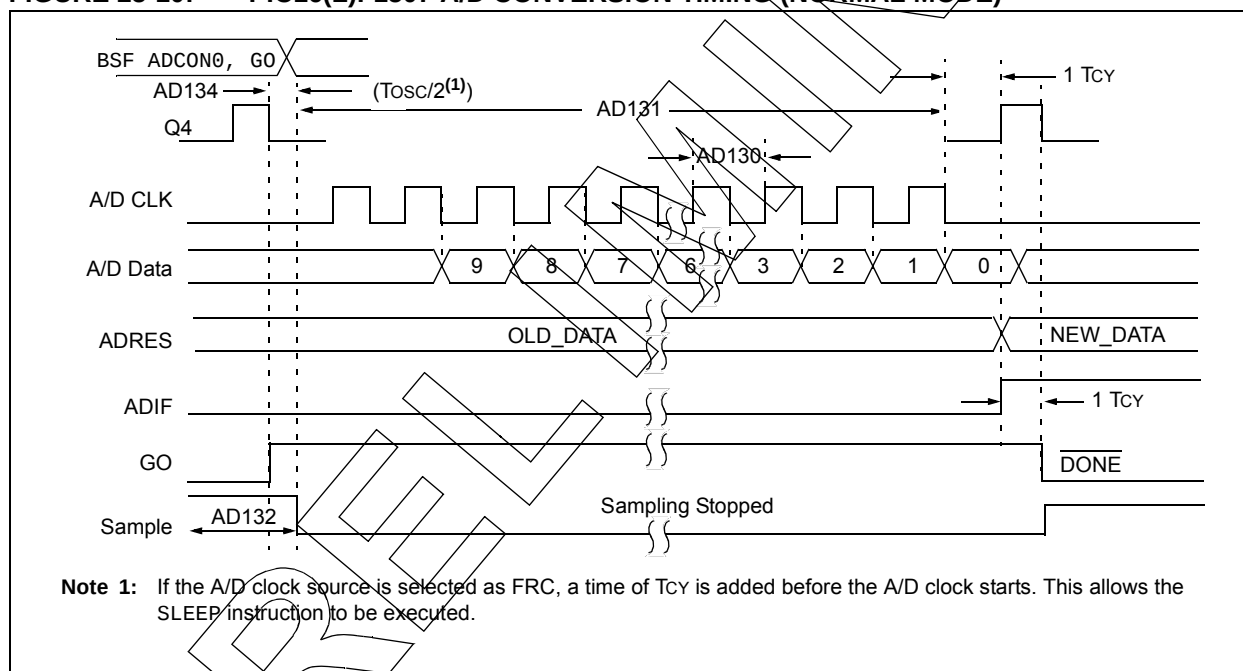
FIGURE 25-10: PIC16(L)F1507 A/D CONVERSION TIMING (NORMAL MODE)
