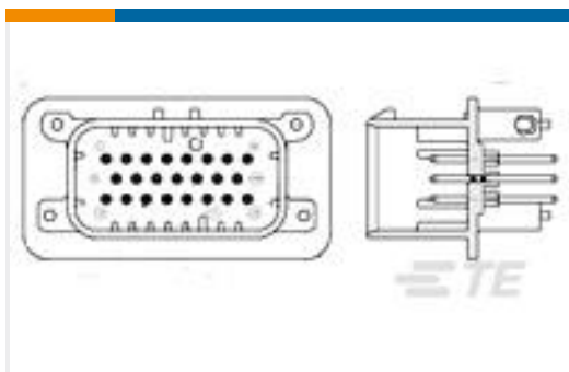
TE 产品编号1-776200-5 HEADER ASSY, 23 POS VERTICAL
