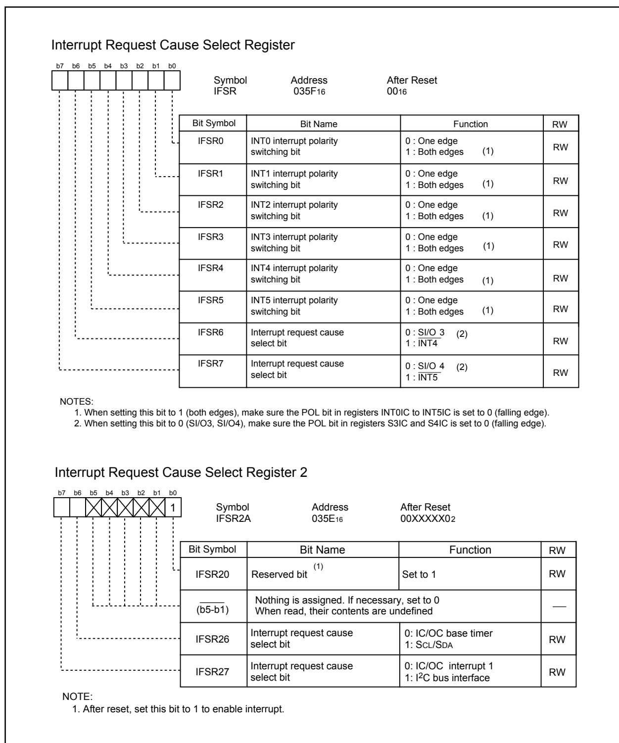
Figure 9.4 IFSR Register and IFSR2A Register
