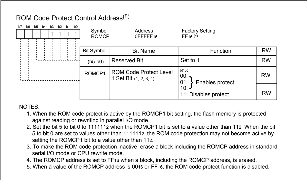
Figure 19.3 ROMCP Address
