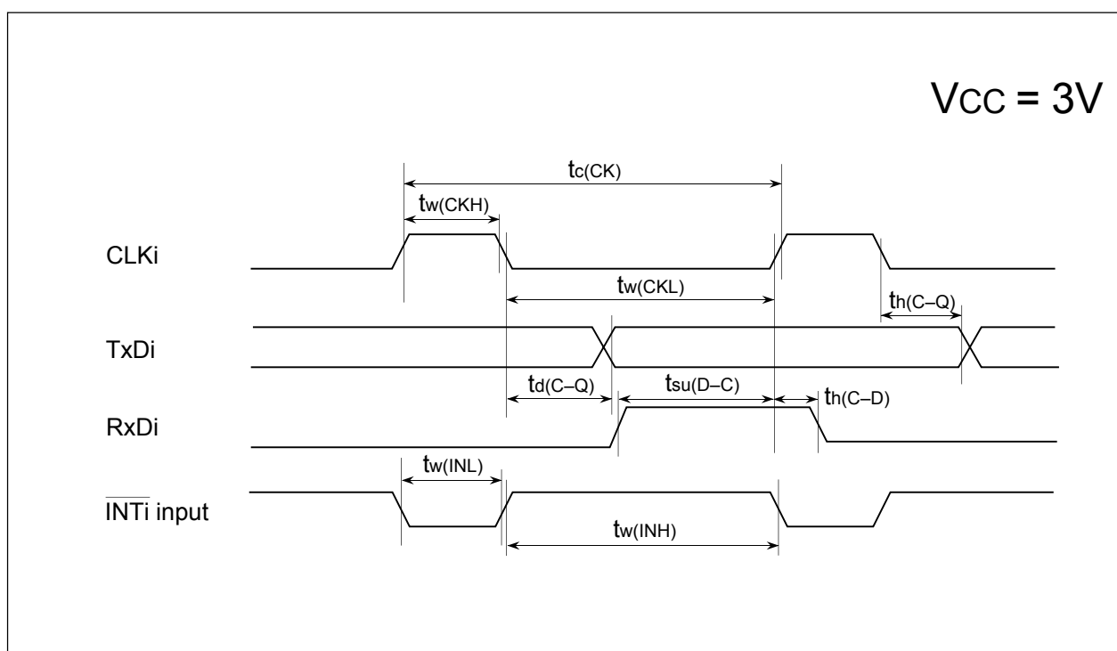
Figure 20.5 Timing Diagram (2)
