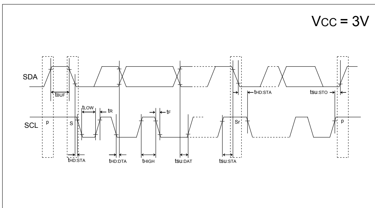
Figure 20.6 Timing Diagram (3)
