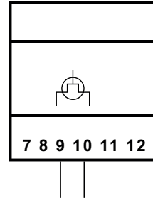
Digital_Output
