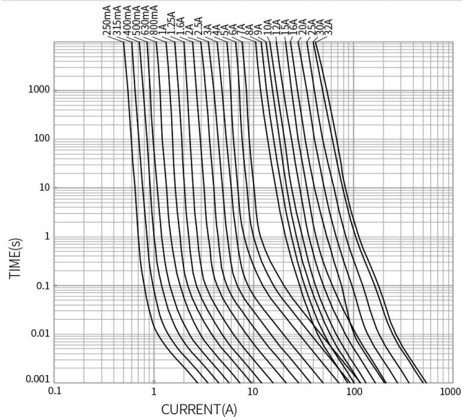
AVERAGE I-T CHARACTERISTICS CURVE (FOR REFERENCE ONLY)
