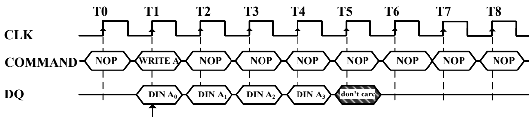
Figure 10. Burst Write Operation (Burst Length = 4)
