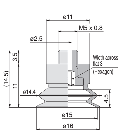
ZP2-TB15MB□-H5
