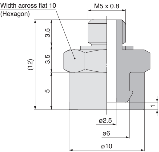
ZP2-T10S□GE-A5
