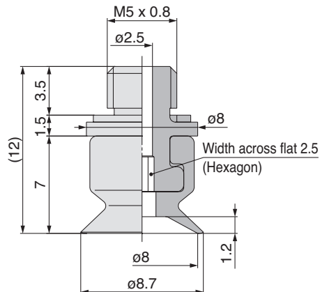
ZP2-TB08MU□-H5
