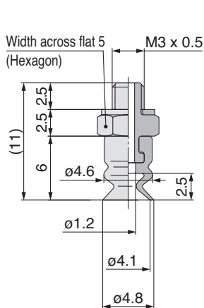
ZP2-TB15MB□-H5
