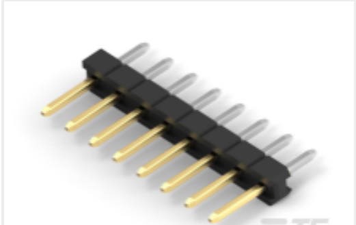
TE Part #2355172-8 8P,2MM,BRK HDR,SRVT,2.8,0.1AU,BOX
