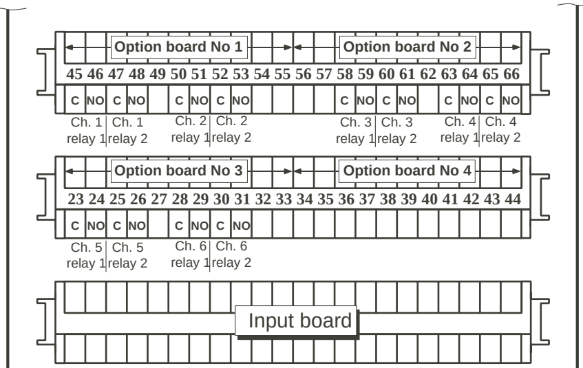
Figure 4.1.2 Normally-open relay wiring (alarm / power off state)
