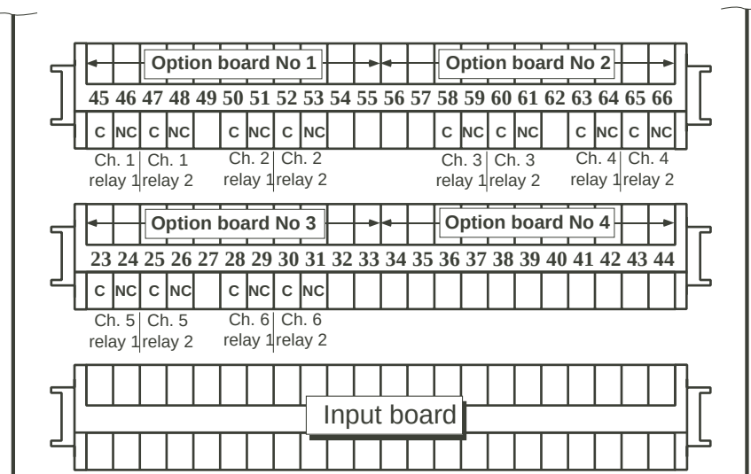
Figure 4.1.3 Normally-closed relay wiring (alarm / power off state)
