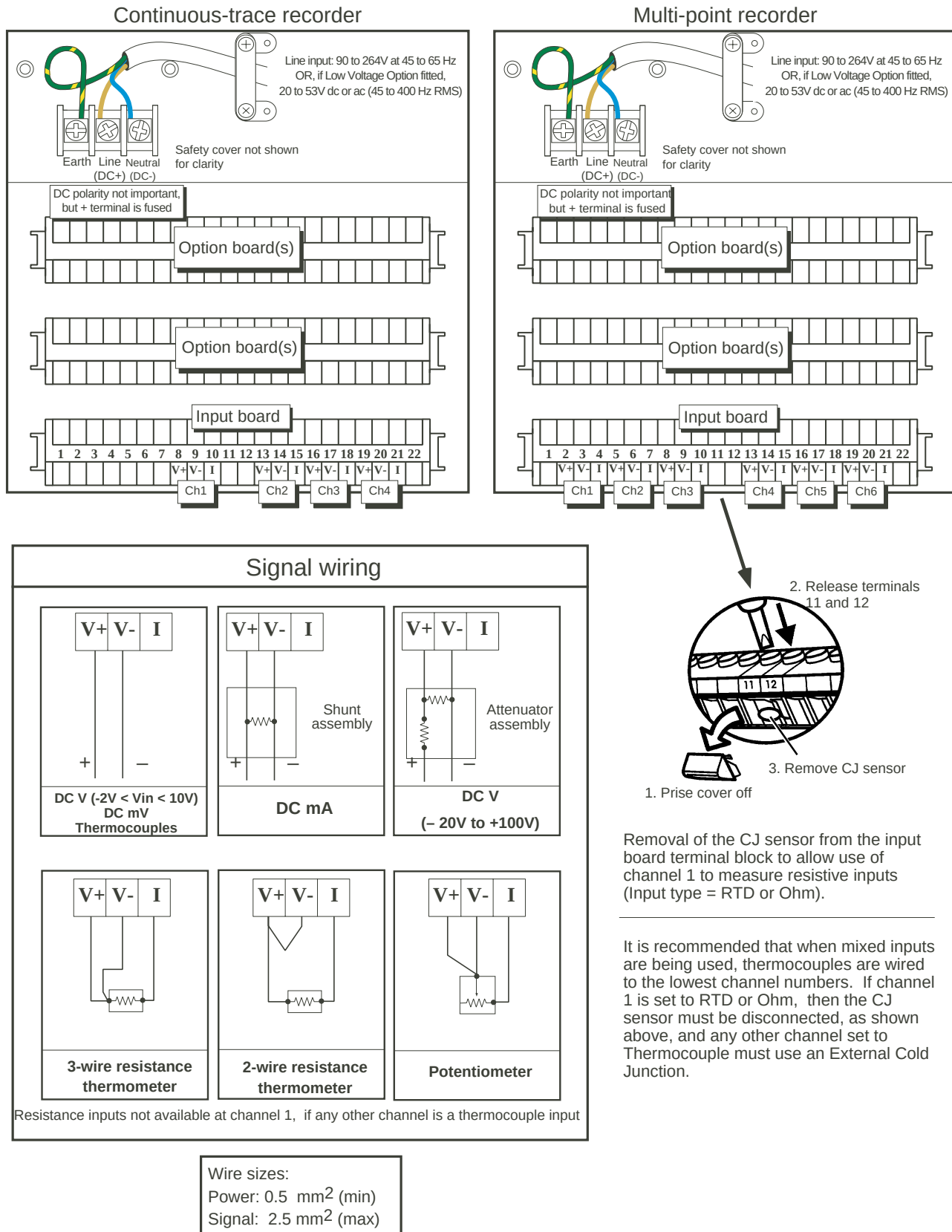
Figure 2.2 Electrical Installation
