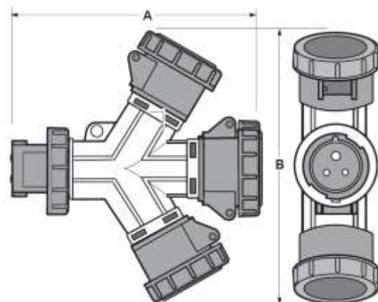
A:285 B:280 Dimensions in mm
