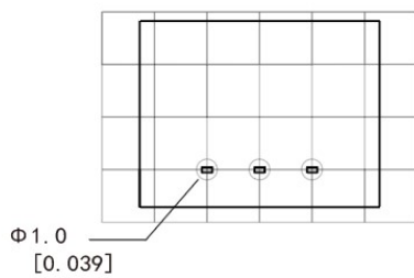
Recommended PCB size diagram
