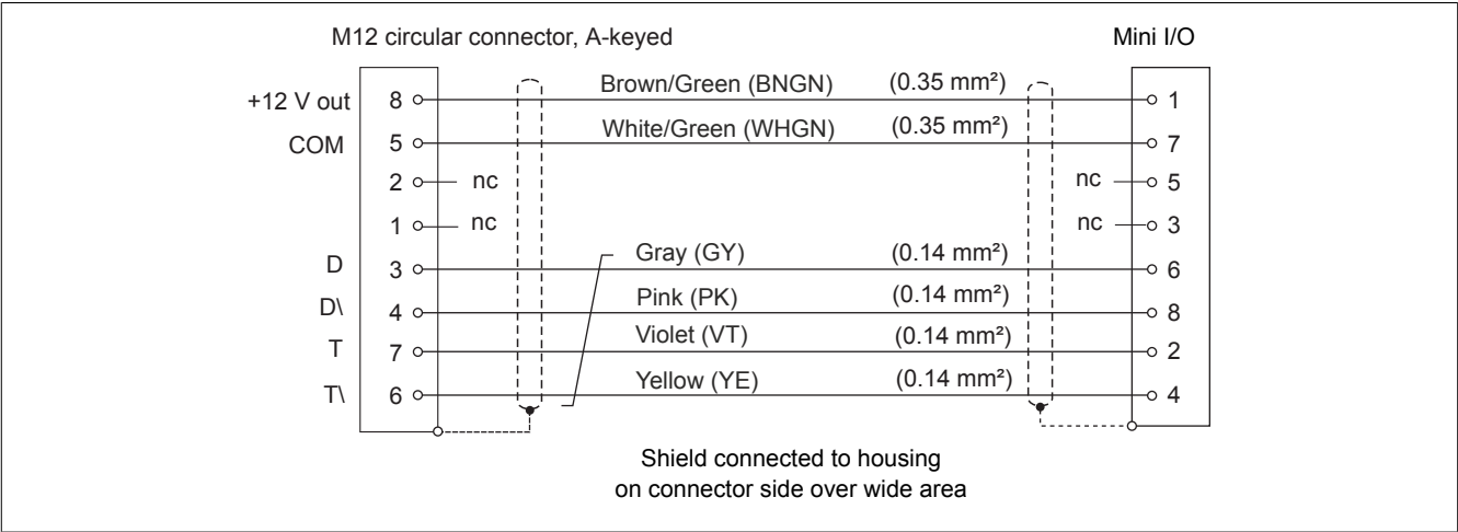
Figure 1: 8ECFxxxx.1231C-0 - Cable diagram
