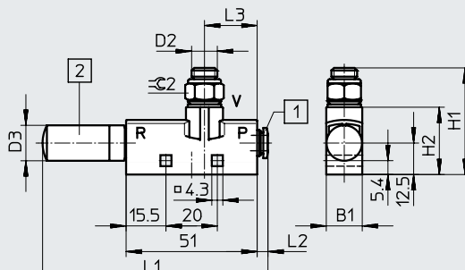
[1] Push-in fitting
