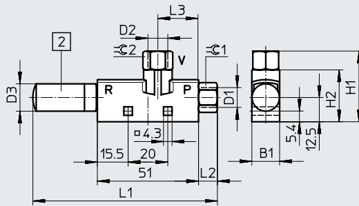
[2] Silencer
