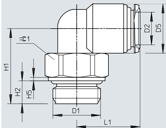
Dimensions – Push-in L-fitting NPQR-L
