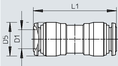
Dimensions – Push-in connector NPQR-D
