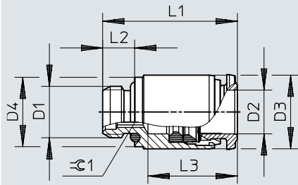
Dimensions – Push-in fitting NPQR-DK-M5/M7/G18/G14
