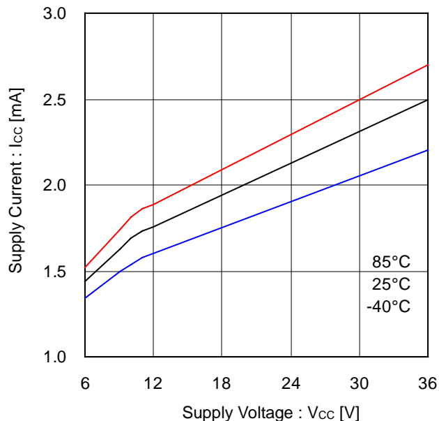
Figure 14. Supply Current vs Supply Voltage (2ch)
