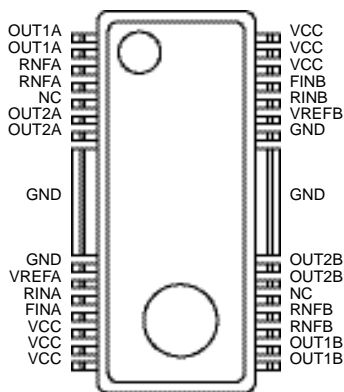
Figure 12. HSOP-M28(TOP VIEW)
