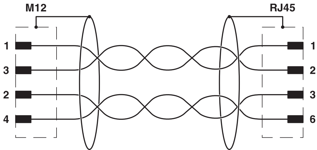
M12和RJ45针式引脚分配
