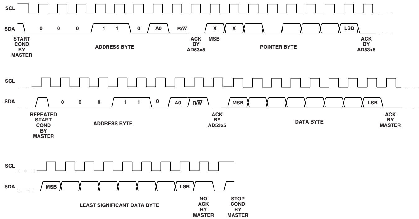
Figure 9. Readback Sequence
