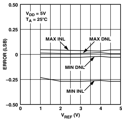
TPC 7. AD5305 INL and DNL Error vs. V_{REF}
