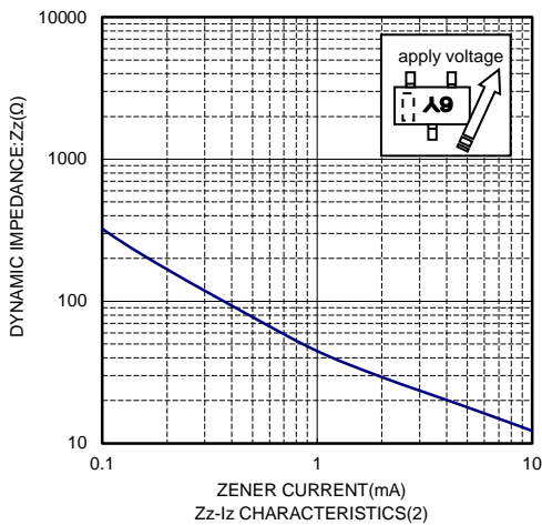
Zz-Iz CHARACTERISTICS(2)
