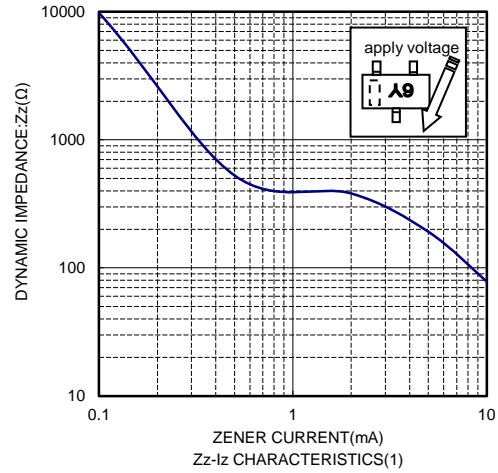
Zz-Iz CHARACTERISTICS(1)
