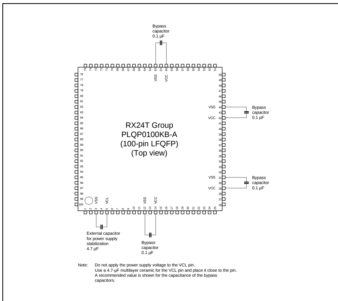
Figure 5.54 Connecting Capacitors (100 Pins)
