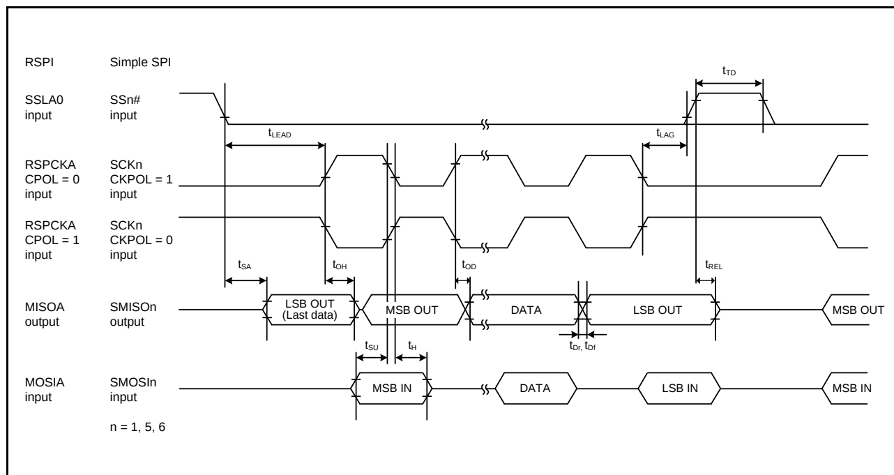
Figure 5.44 RSPI Timing (Slave, CPHA = 1) and Simple SPI Clock Timing (Slave, CKPH = 0)
