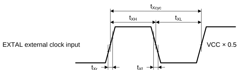
Figure 5.20 EXTAL External Clock Input Timing
