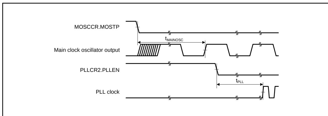
Figure 5.24 PLL Clock Oscillation Start Timing (PLL is Operated after Main Clock Oscillation Has Settled)
