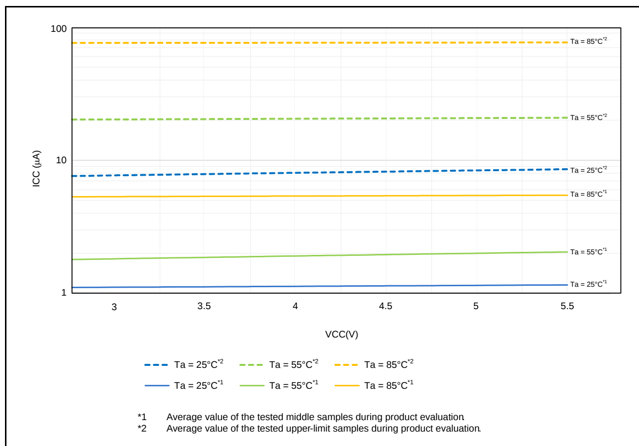
Figure 5.1 Voltage Dependency in Software Standby Mode (Reference Data)
