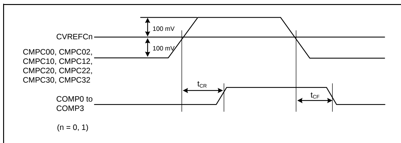
Figure 5.47 Comparator Response Time
