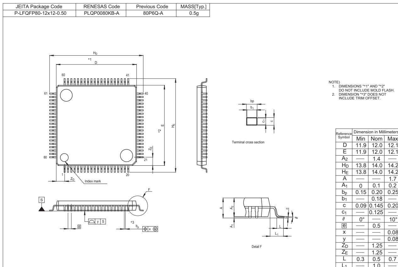
Figure C 80-Pin LFQFP (PLQP0080KB-A)
