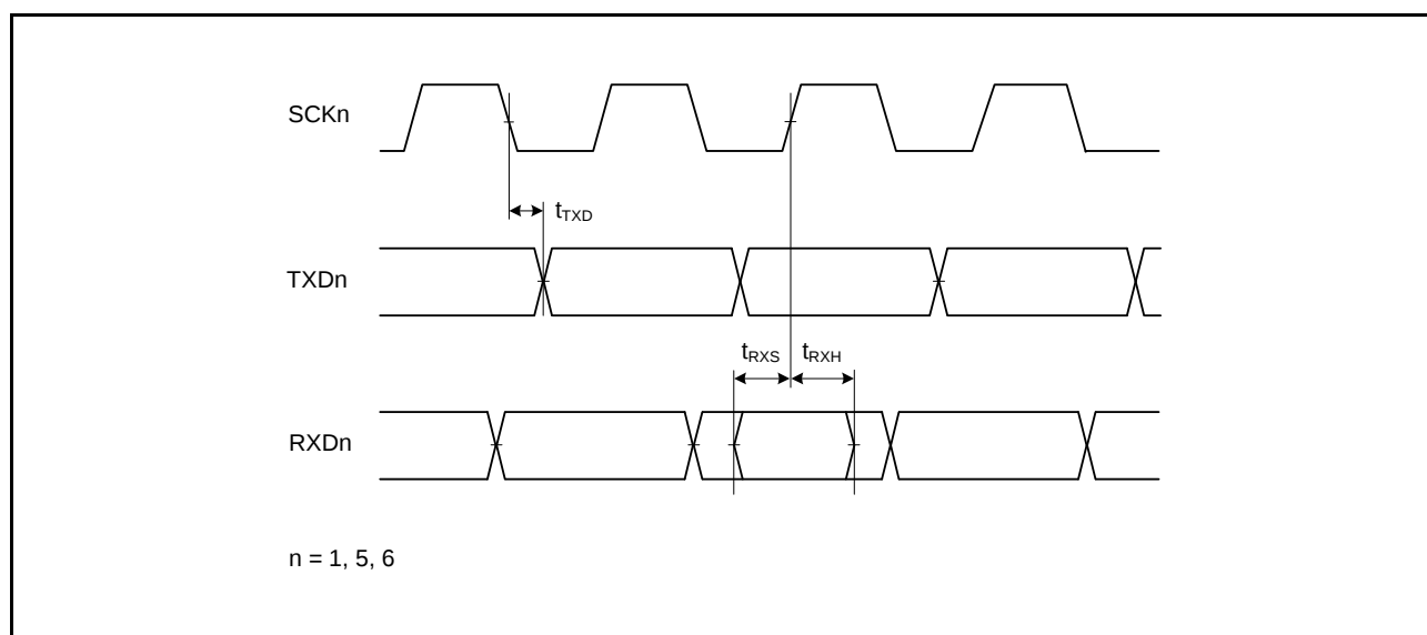
Figure 5.38 SCI Input/Output Timing: Clock Synchronous Mode
