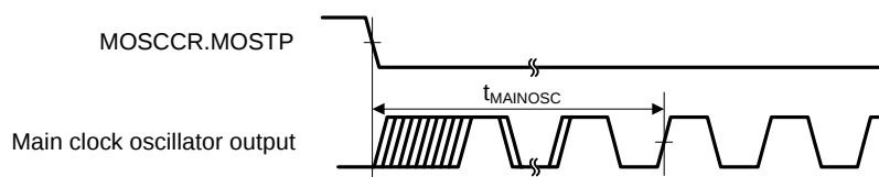
Figure 5.21 Main Clock Oscillation Start Timing
