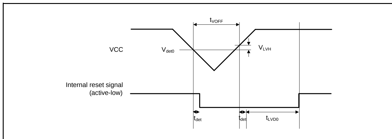
Figure 5.50 Voltage Detection Circuit Timing (Vdet0)
