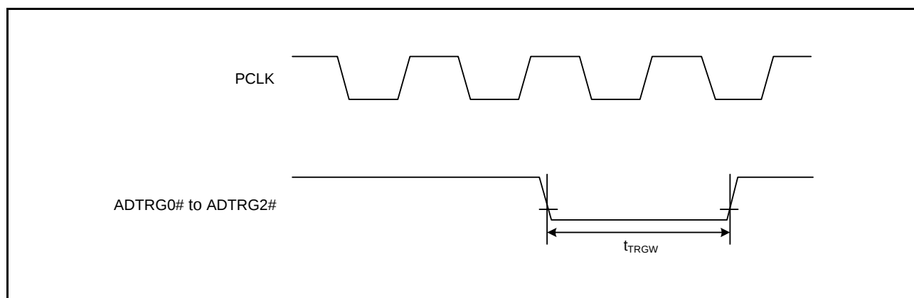
Figure 5.39 A/D Converter External Trigger Input Timing
