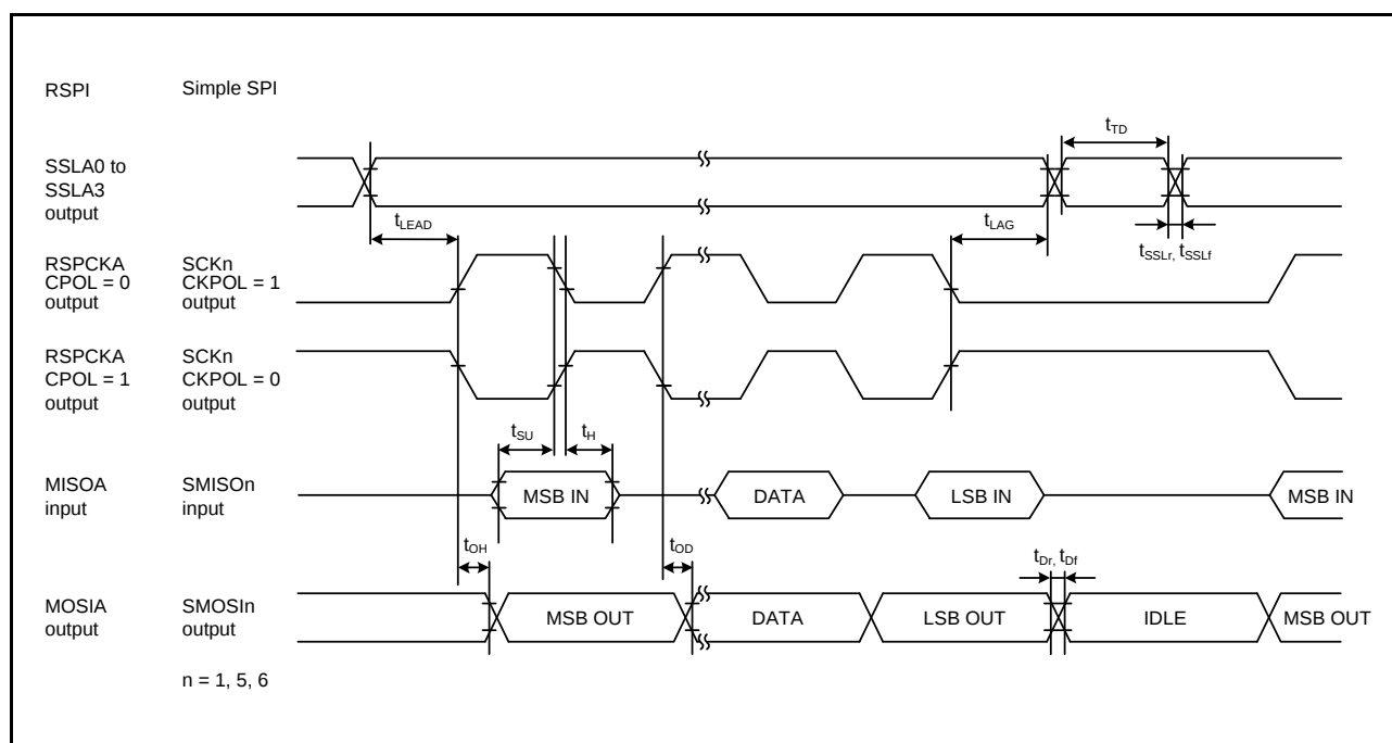
Figure 5.42 RSPI Timing (Master, CPHA = 1) and Simple SPI Clock Timing (Master, CKPH = 0)
