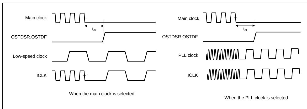
Figure 5.53 Oscillation Stop Detection Timing
