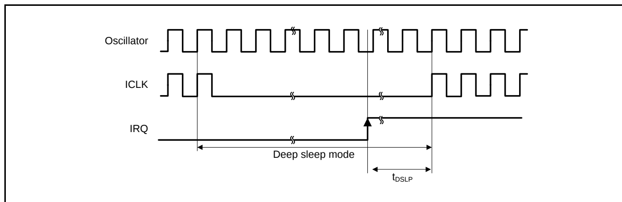
Figure 5.29 Deep Sleep Mode Recovery Timing
