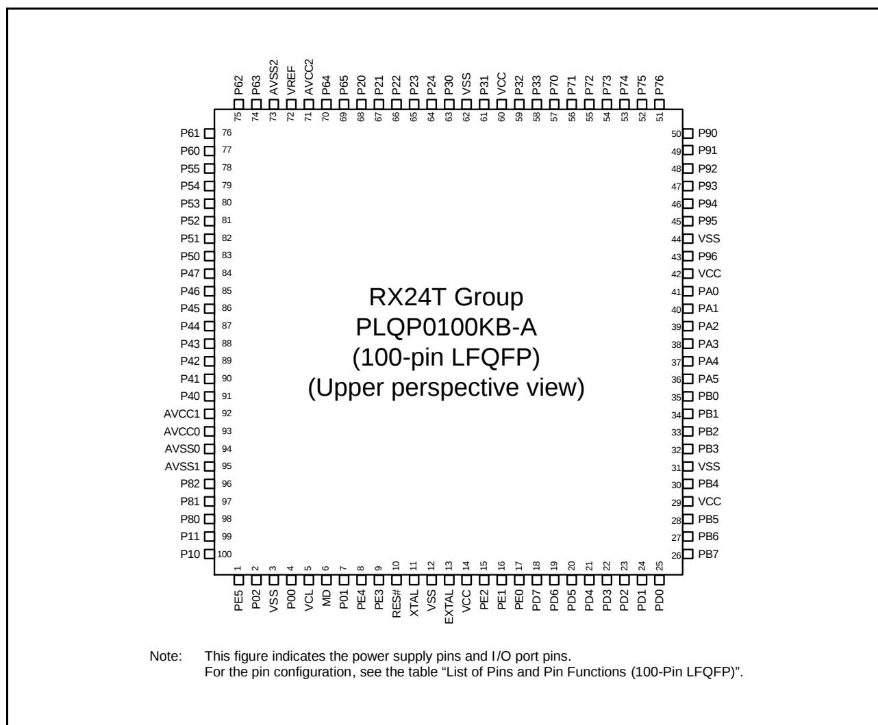
Figure 1.3 Pin Assignments of the 100-Pin LFQFP
