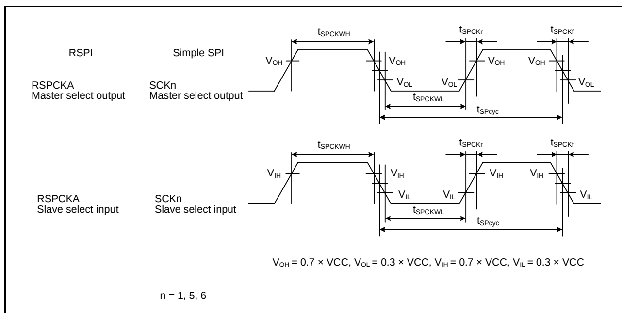
Figure 5.40 RSPI Clock Timing and Simple SPI Clock Timing
