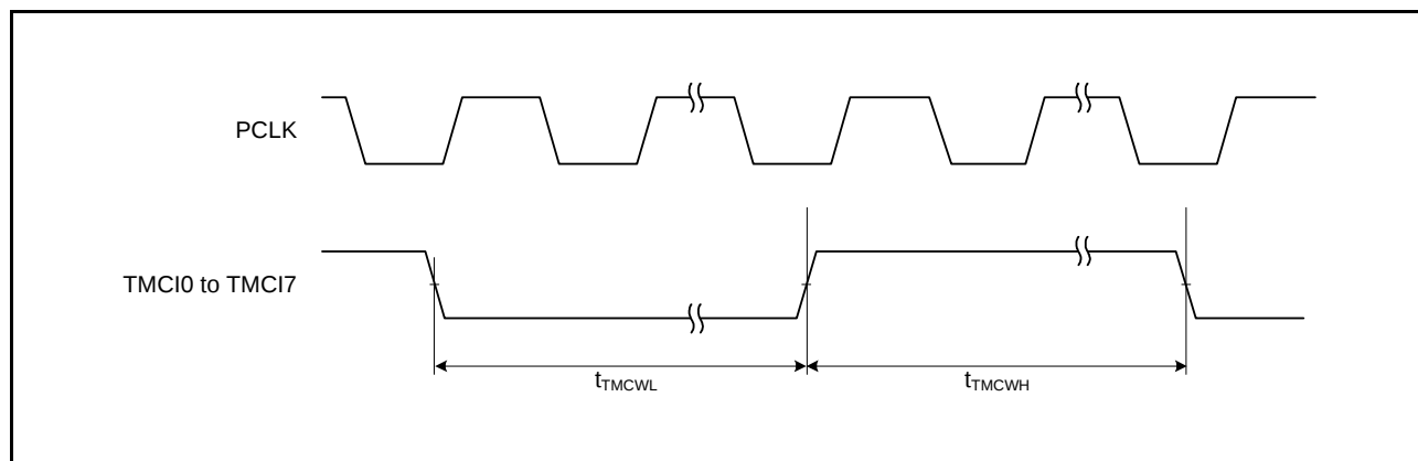
Figure 5.36 TMR Clock Input Timing
