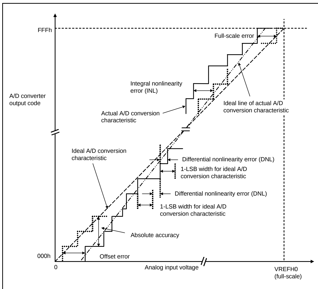
Figure 5.46 Illustration of A/D Converter Characteristic Terms
