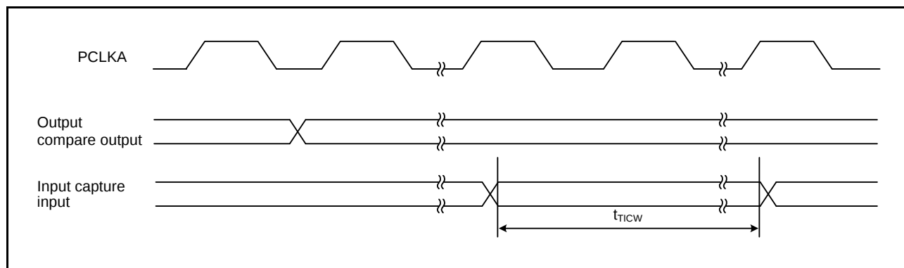
Figure 5.33 MTU3 Input/Output Timing
