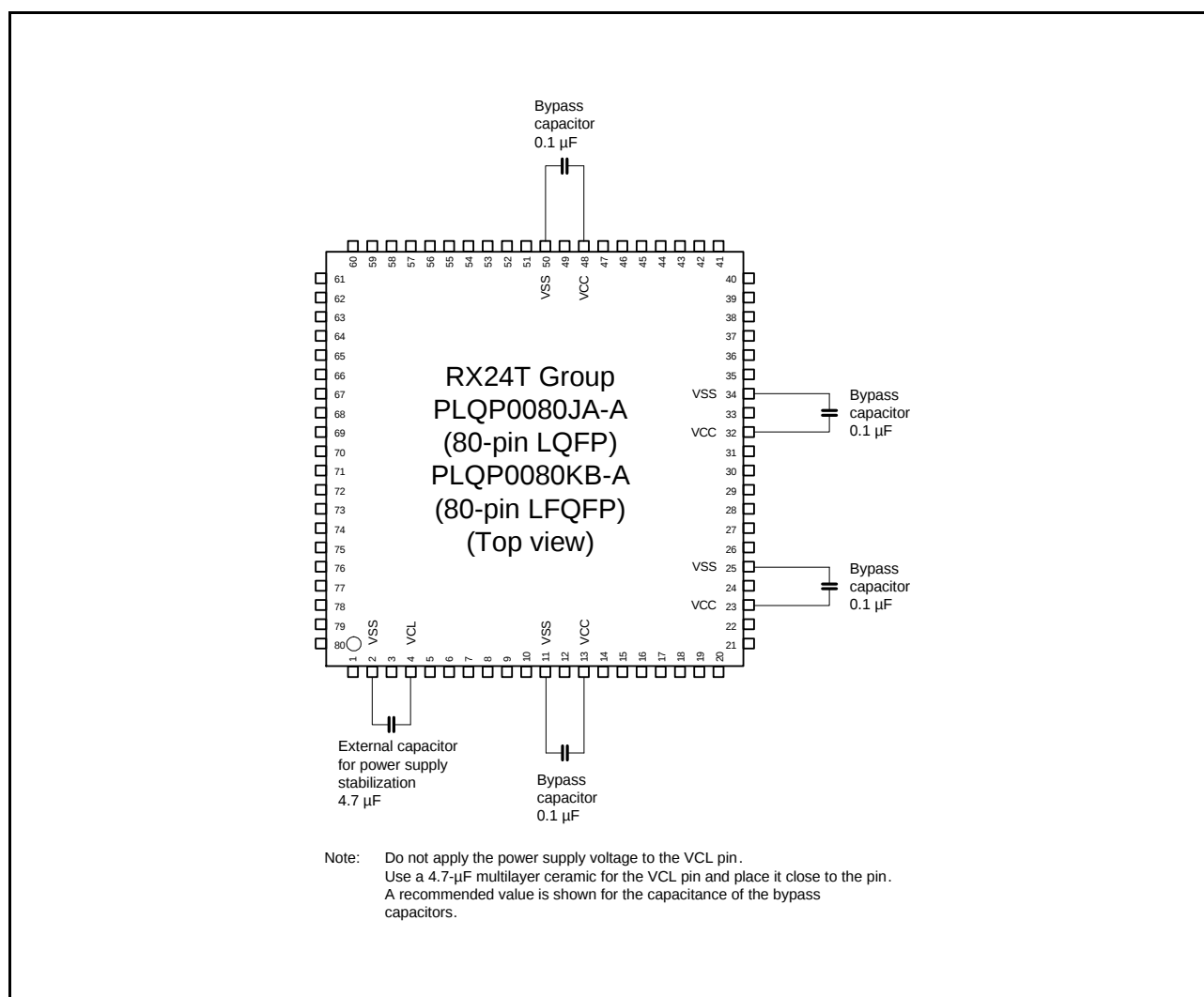
Figure 5.55 Connecting Capacitors (80 Pins)
