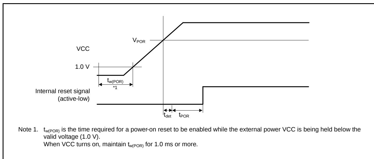
Figure 5.49 Power-On Reset Timing
