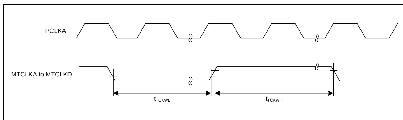
Figure 5.34 MTU3 Clock Input Timing
