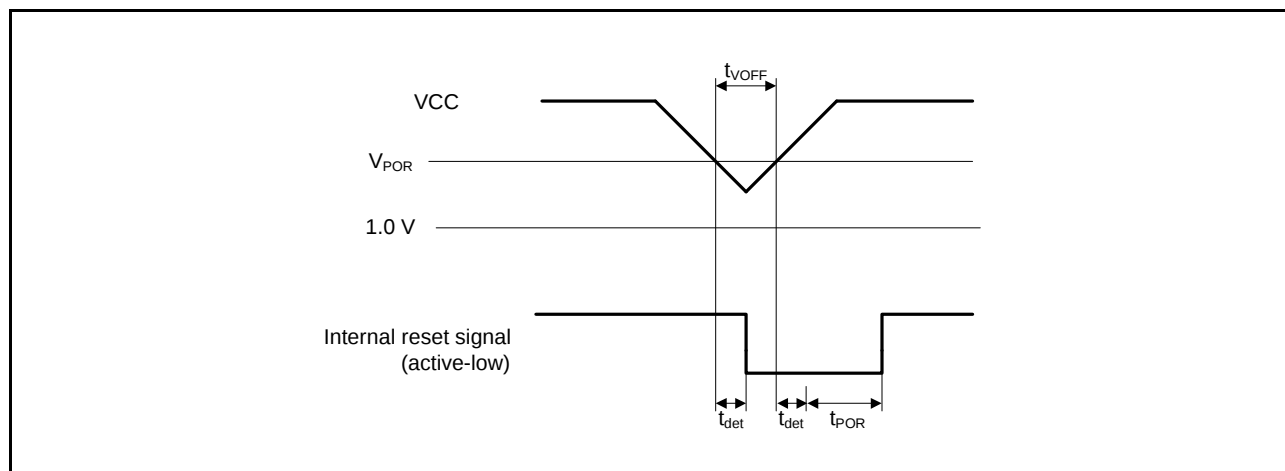
Figure 5.48 Voltage Detection Reset Timing
