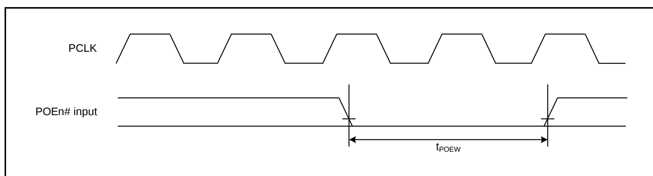
Figure 5.35 POE# Input Timing
