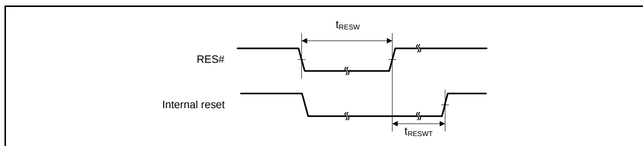
Figure 5.26 Reset Input Timing (1)
