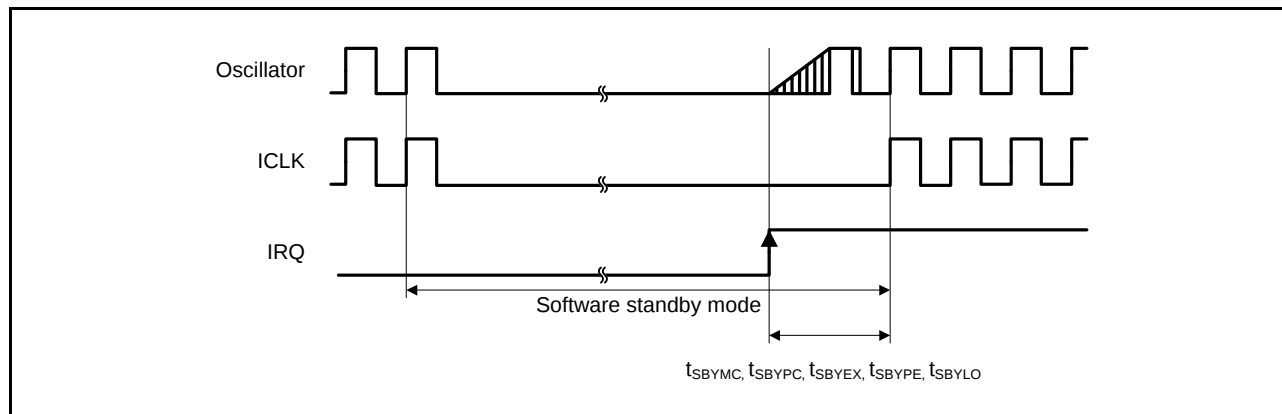
Figure 5.28 Software Standby Mode Recovery Timing
