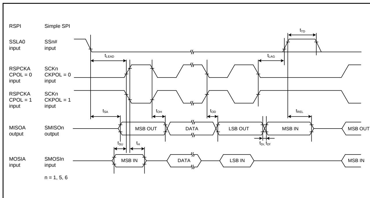
Figure 5.43 RSPI Timing (Slave, CPHA = 0) and Simple SPI Clock Timing (Slave, CKPH = 1)
