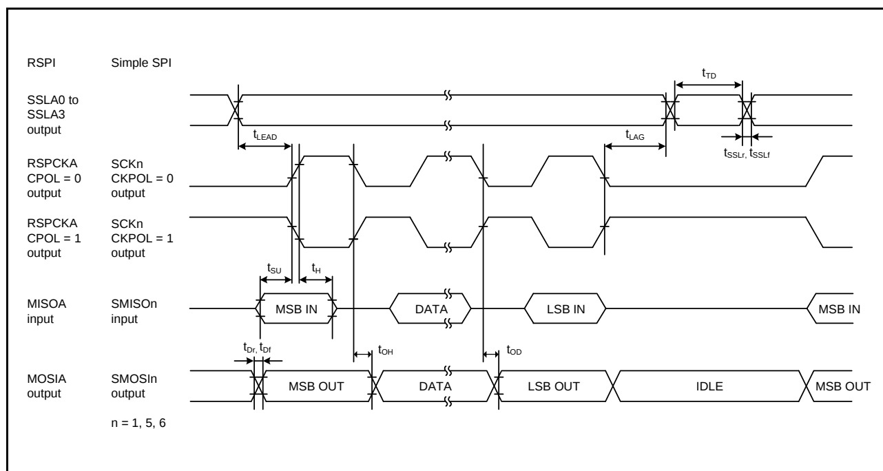
Figure 5.41 RSPI Timing (Master, CPHA = 0) and Simple SPI Clock Timing (Master, CKPH = 1)
