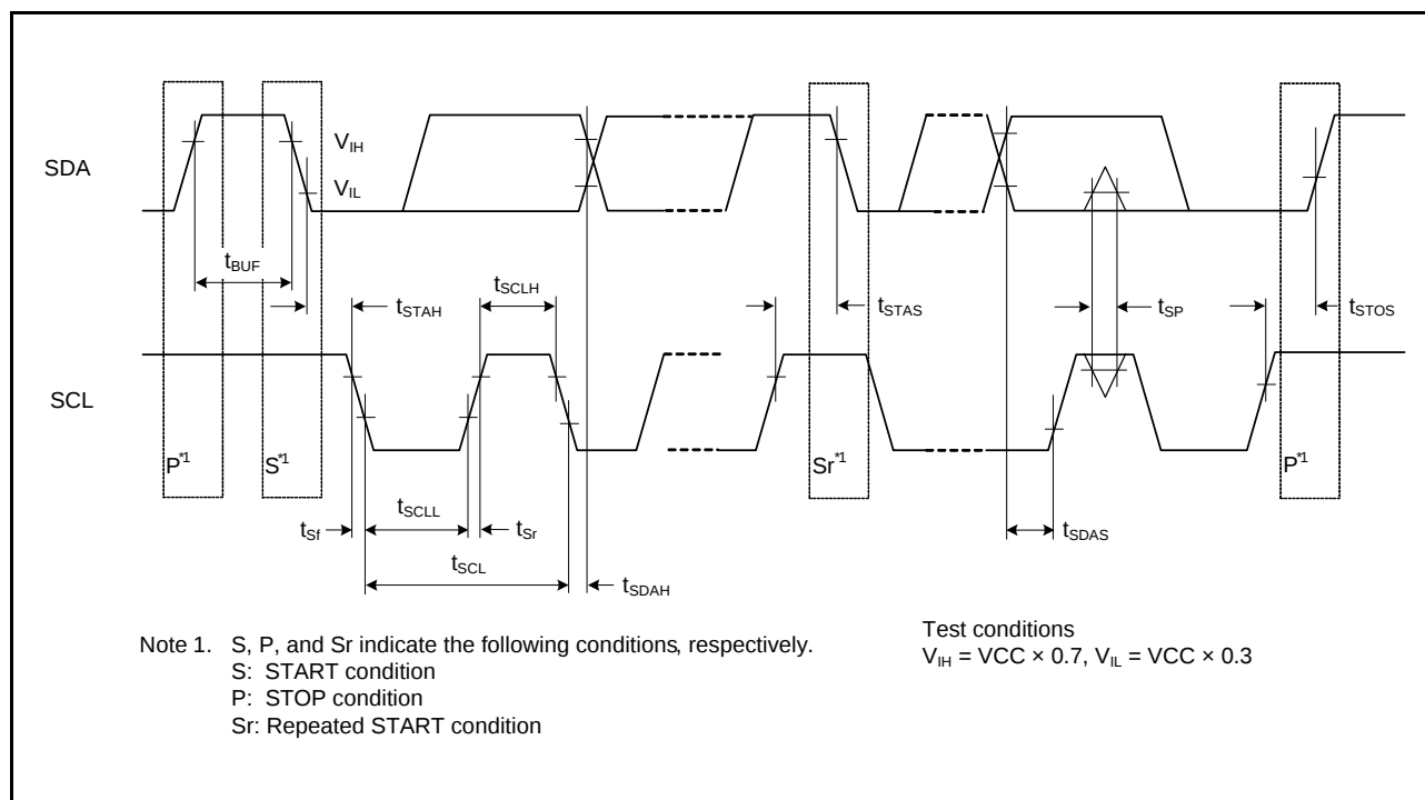
Figure 5.45 IIC Bus Interface Input/Output Timing and Simple I2C Bus Interface Input/Output Timing
