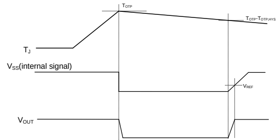
Figure 11. Overtemperature protection
