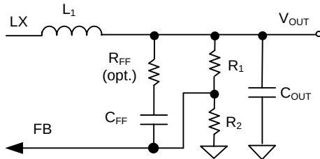
Figure 13. Feed-forward network
