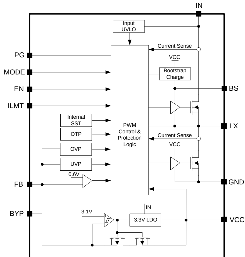
Figure 3. Block Diagram
