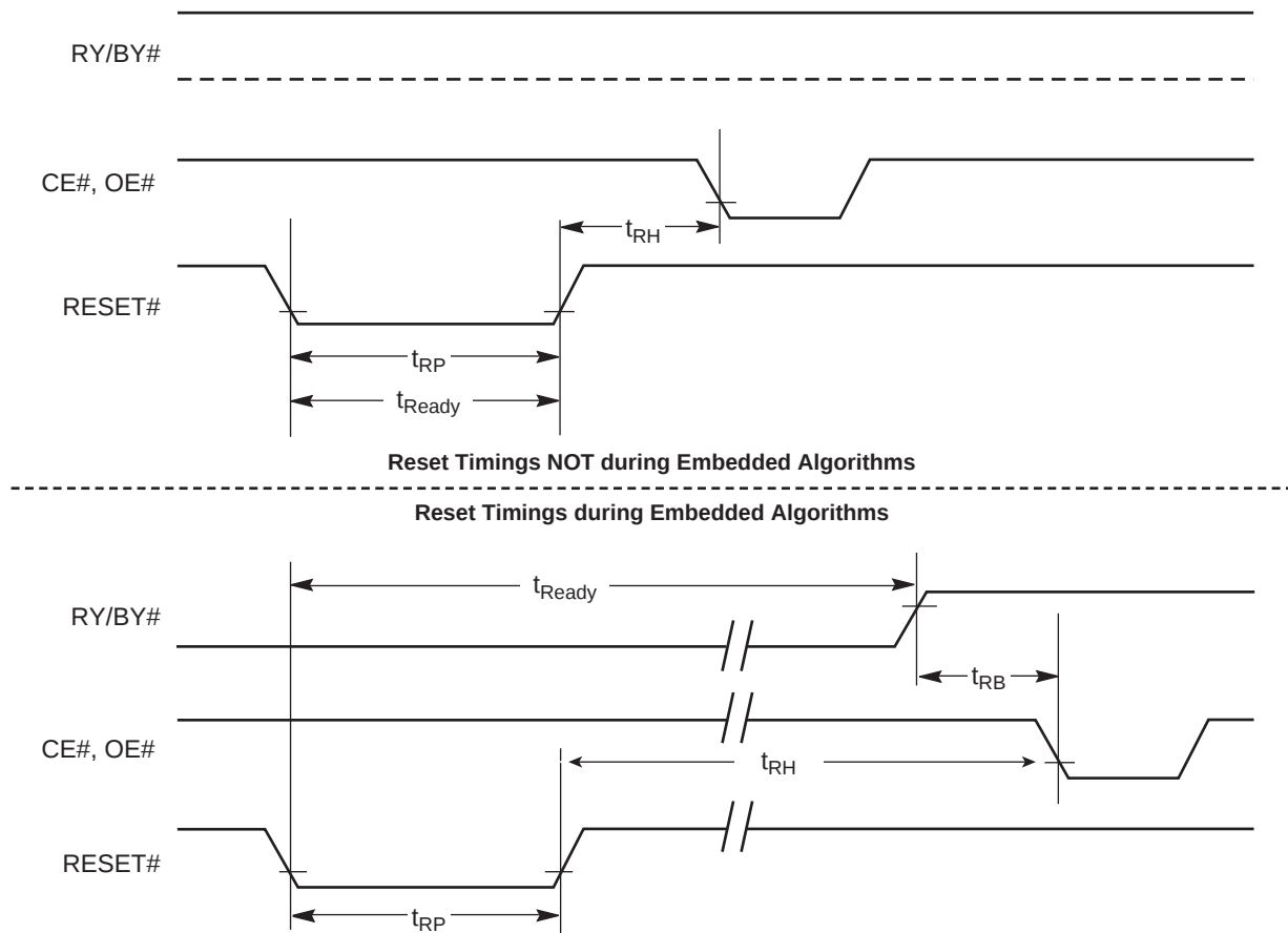
Figure 15.4 Reset Timings
