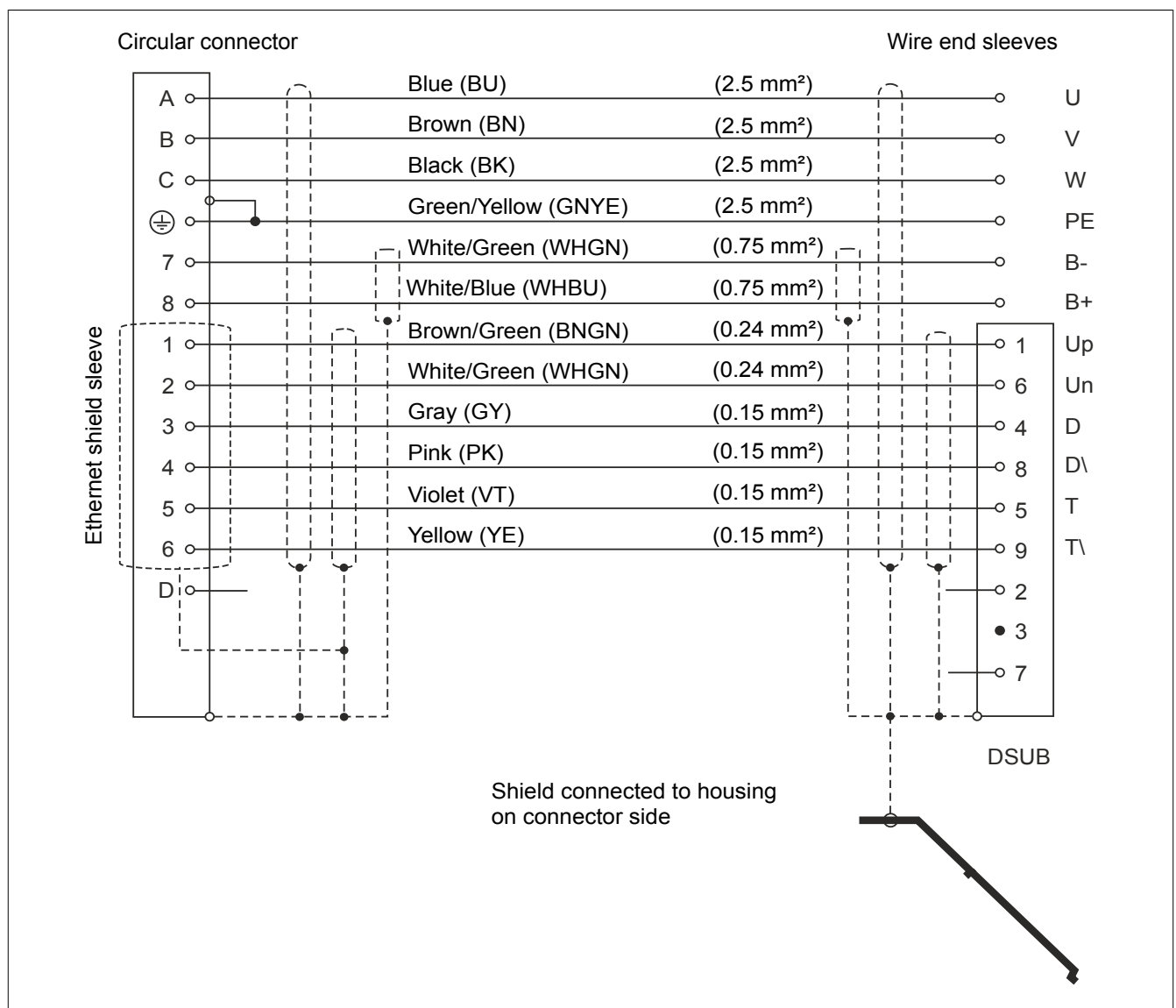
Figure 1: 2.5 mm 2 food-grade hybrid motor cables - Cable diagram
